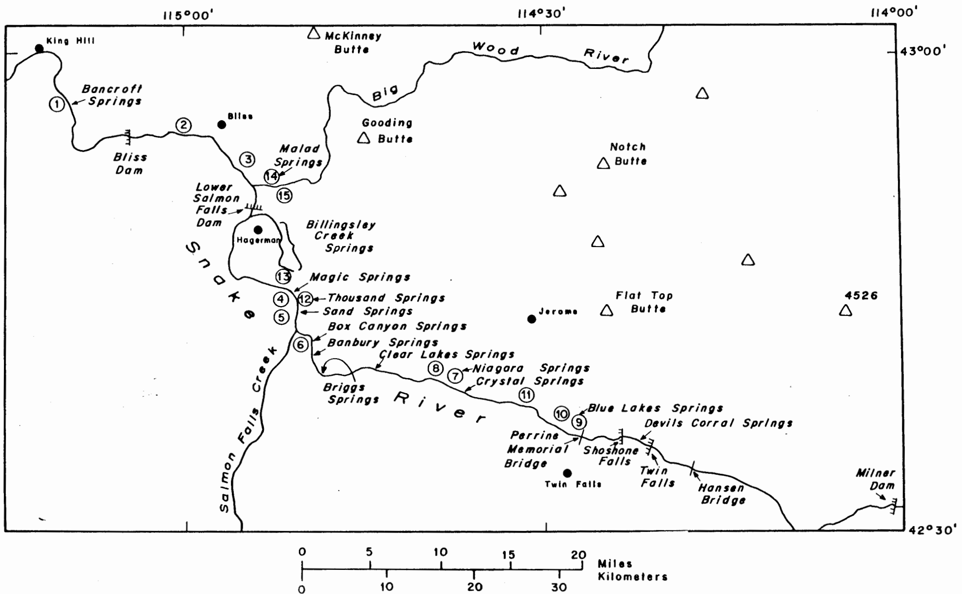
FIGURE 2.--Map showing major physiographic features of the field trip area, and numbered locations of field trip stops.
