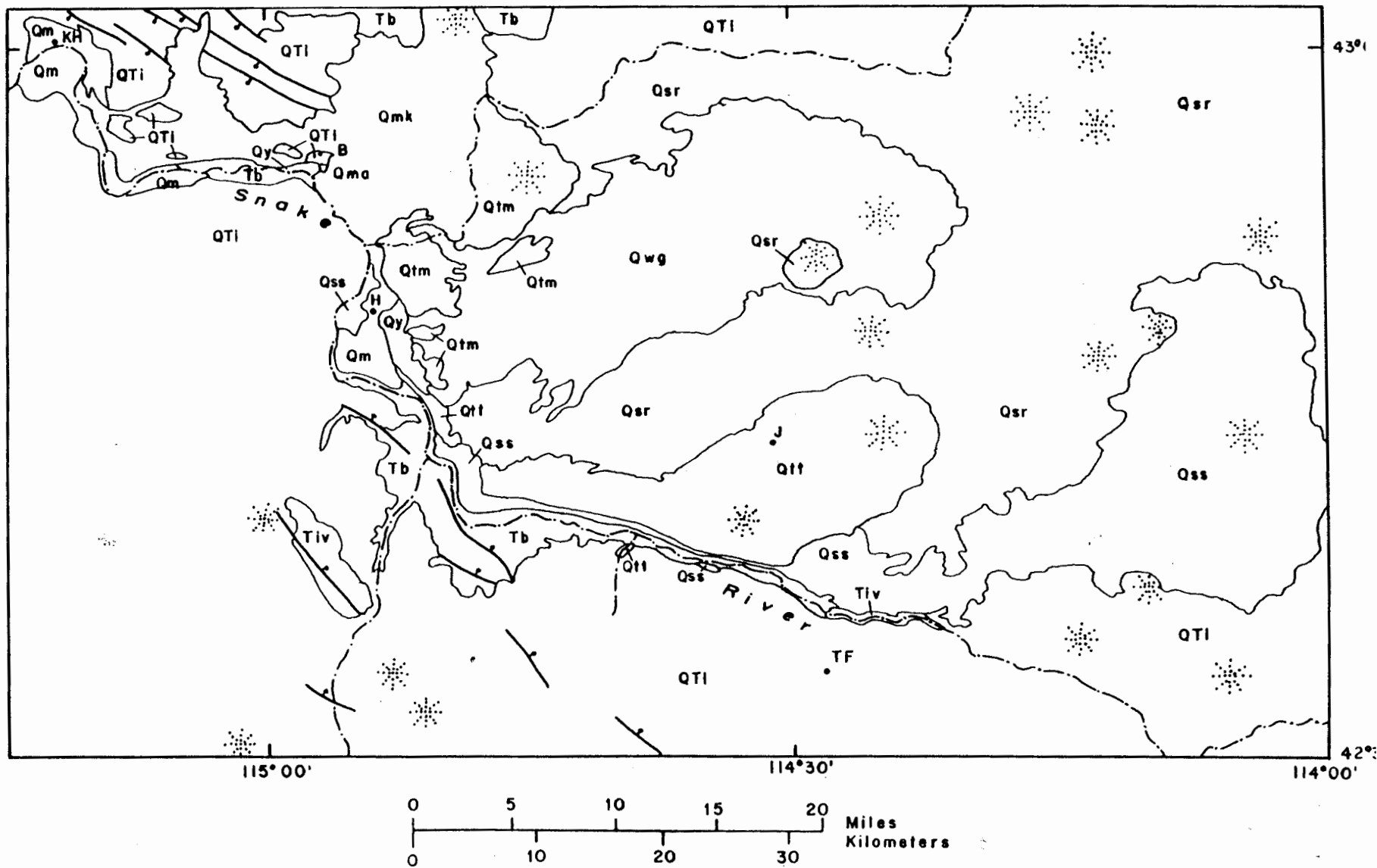
FIGURE 5.--Generalized geologic map of the field trip area. (B) Bliss, (H) Hagerman, (J) Jerome, (KH) King Hill, (TF) Twin Falls. Modified from Malde and others (1963).
