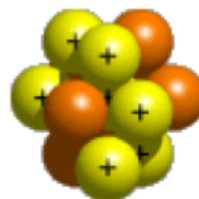
Nitrogen-14
