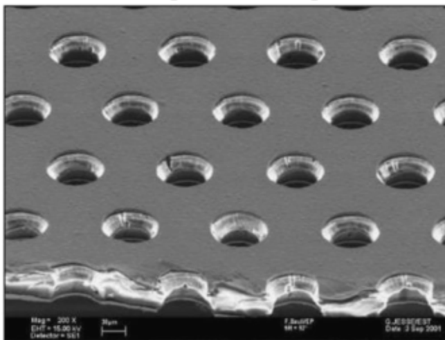
GEM foil perforation pattern:
