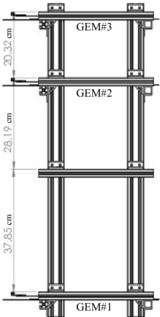
Aluminum ladder-frame
