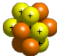
Carbon-14
